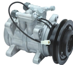
VW OEM#:82292901/8FK351339721 TYPE: 10PA17C PULLEY: A1 120mm VOLTAGE: 12V
