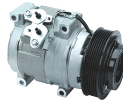
Car Model: TOYOTA FORTUNER OEM#: 88320-35730/4472205270 TYPE: 10S15C PULLEY: 7PK 125mm VOLTAGE: 12V
