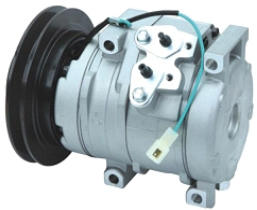
TYPE: 10S15C OEM#: PULLEY: A1 142mm VOLTAGE: 24V
