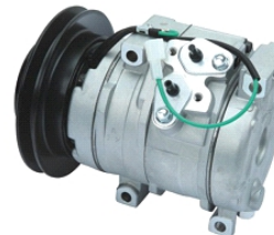
HINO TRUCK OEM#: TYPE: 10S15C PULLEY: A1 142mm VOLTAGE: 24V
