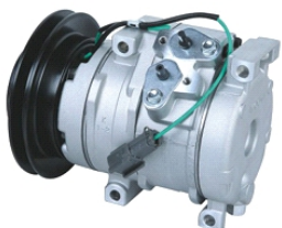
KOMATSU-7 OEM#: TYPE: 10S15C PULLEY: A1 142mm VOLTAGE: 24V
