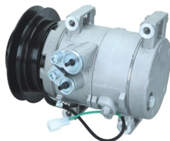
GAC HINO OEM#: TYPE: 10PA15C PULLEY: B1 138mm VOLTAGE: 24V
