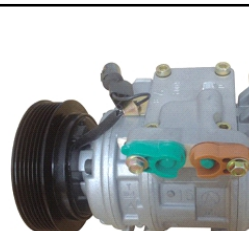
FORTE OEM#: TYPE: 10PA15C PULLEY: 6PK 128mm VOLTAGE: 12V
