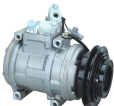
LAND CRUISER OEM#: TYPE: 10PA20C PULLEY: A1 135mm VOLTAGE: 12V
