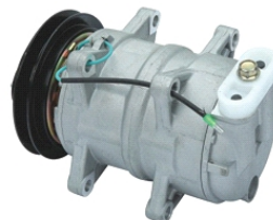
DELICA EQ OEM#: TYPE: DKS17C PULLEY: A1 135mm VOLTAGE: 12V
