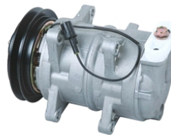
FREECA OEM#: TYPE: DKS17 PULLEY: A1 135mm VOLTAGE: 12V
