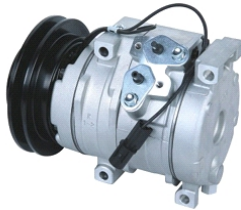
ENGINEERING TRUCK OEM#: TYPE: 10S15C PULLEY: A1 133.8mm VOLTAGE: 12V
