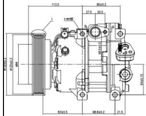
HYUNDAI SONATA 3.3(08-10) OEM#97701-3K425 TYPE#VS16 PULLEY#BPK125mm
