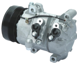
SUZUKI OEM#: TYPE: 6SEU14C PULLEY: PV5 110mm VOLTAGE: 12V
