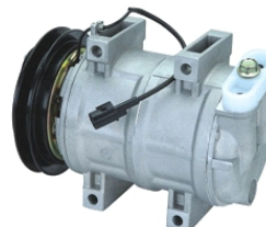
MITSUBISHI L200 OEM#: TYPE: DKS PULLEY: A1 VOLTAGE: 12V
