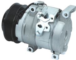
TOYOTA INNOVA GASOLINE OEM#: TYPE: 10S15C PULLEY: 7PK 125mm VOLTAGE: 12V
