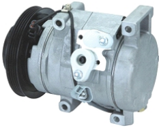
TOYOTA V2700 WITHSPEED SENSING OEM#: TYPE: 10S17C PULLEY: 4PK 136mm VOLTAGE: 12V
