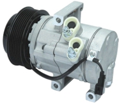
FORD PICKUP OEM#:140595/1715092 TYPE:10S12 PULLEY: 7PK 109mm VOLTAGE: 12V
