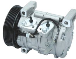
SUZUKI OEM#: TYPE: 10S11C PULLEY: 6PK 110mm VOLTAGE: 12V
