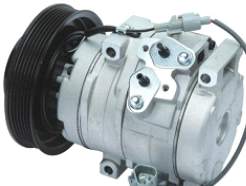
TOYOTA COROLLA OEM#: TYPE: 10S15C PULLEY: 6PK 140mm VOLTAGE: 12V
