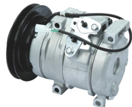
ENGINEERING TRUCK OEM#: TYPE: 10S15C PULLEY: B1 142mm VOLTAGE: 24V
