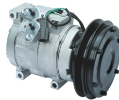
KOMATSU OEM#: TYPE: 10S15C PULLEY: B1 152mm VOLTAGE: 24V
