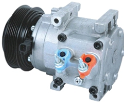
FORD OEM#: TYPE: HS15 PULLEY: 6PK 120mm VOLTAGE: 12V
