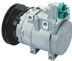
FORD OEM#:CS20524 TYPE: HS15 PULLEY: A1 142mm VOLTAGE: 12V
