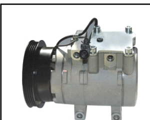
KIA RIO OEM#:140141/97701-25000 TYPE: HS15 PULLEY: 4PK 129mm VOLTAGE: 12V
