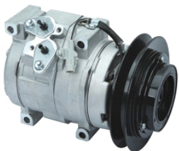
HINO TRUCK OEM#: TYPE: 10S15C PULLEY: B1 142mm VOLTAGE: 24V
