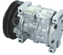
SUZUKI OEM#: TYPE: 10S13C PULLEY: A1 135mm VOLTAGE: 12V
