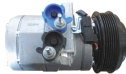
FORD OEM#: TYPE: FS20 PULLEY: 6PK 125mm VOLTAGE: 12V
