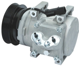
FORD FIESTA OEM#: TYPE: FS15 Grooves: PV6 PULLEY: 6PK 119mm VOLTAGE: 12V
