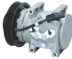
FORD OEM#:RC.600.106 TYPE: SH15 PULLEY: 6PK 143mm VOLTAGE: 12V
