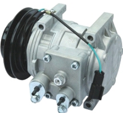
ENGINEERING TRUCK OEM#: TYPE: 10PA15C PULLEY: A1 125mm VOLTAGE: 24V
