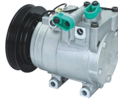
LIONCEL OEM#: TYPE: HCC PULLEY: 5PK 137mm VOLTAGE: 12V
