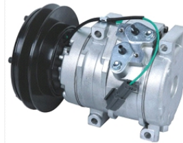
ENGINEERING TRUCK OEM#: TYPE: 10S15C PULLEY: B1 152mm VOLTAGE: 24V
