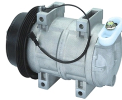
MITSUBISHI CHEETAH OEM#: TYPE: DKS PULLEY: 4PK VOLTAGE: 12V
